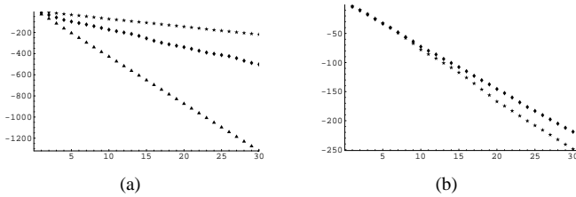
Fig. 2. Plot (a) shows the progression of \mathcal{H}^{(k)} as k increases, resulting from the static (triangle), lawnmower (diamond), and gradient descent (star) approaches. For the gradient descent algorithm only, plot (b) compares the value of \tilde{\mathcal{E}} (stars) against the approximation, \mathcal{H}^{(k)} (diamonds).
