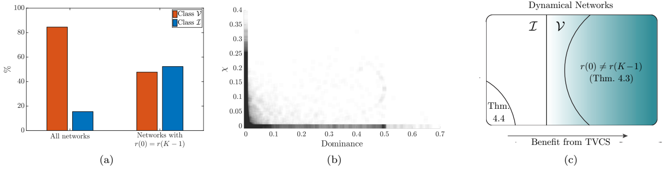
Figure 3: The role of 2k -communicability in distinguishing between networks of class \mathcal{V} ( \chi > 0 ) and \mathcal{I} ( \chi = 0 ). (a) The proportion of random networks in \mathcal{V} and \mathcal{I} . A total of 10^5 random connectivity matrices were generated with logarithmically-uniform n in [10^1, 10^3] , uniform sparsity p in [0, 1] , and uniform pairwise connectivity weight in [0, 1] , and then transformed to adjacency matrices A using the transmission method (cf. Appendix A). A time-horizon of K = 10 is used for all networks. While more than 80% of all networks belong to class \mathcal{V} , this number drops to less than 50% among networks with r(1) = r(K-1) (i.e., networks where the same node has the greatest local and global centralities). (b) The \chi -value of the same networks as in (a) that have r(1) = r(K-1) as a function of the dominance of the node r(0) . For the node r(0) , its dominance (over the rest of the network) is a measure of how distinctly R_{r(0)}(1) and R_{r(0)}(K-1) are larger than R_i(1) and R_i(K-1) , respectively, for i \neq r(0) (cf. Appendix D). Each gray square represents one randomly generated network, so the darkness of each area represents the probability of observing random networks with that value of (dominance, \chi ). A rapid decay of \chi with dominance is clear, such that networks with positive dominance have very low probability of having \chi > 0 . (c) A Venn diagram illustrating the decomposition of dynamical networks based on the extent to which they benefit from TVCS. The color gradient is a depiction of this extent, as measured by \chi (equation (6)), where darker areas correspond to higher \chi . As shown in (a) and (b), the class of networks for which r(0) \neq r(K-1) is only a subset of \mathcal{V} but provides a good approximation for it.
