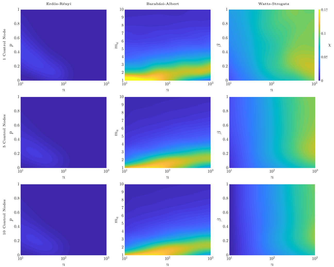
Figure 9: Average value of \chi for networks with increasing number of inputs. The plots show the effect of multiple inputs on TVCS. The details on how to obtain the plots are similar to Figure 6 in the main text. The dynamic adjacency matrix A is obtained from the raw static connectivity C using the transmission method in all cases. These plots show a slight depression in the benefit of TVCS as the number of control nodes grows, despite the fact that networks with more control nodes have a higher probability of belonging to \mathcal{V} (namely, having \chi > 0 ).
