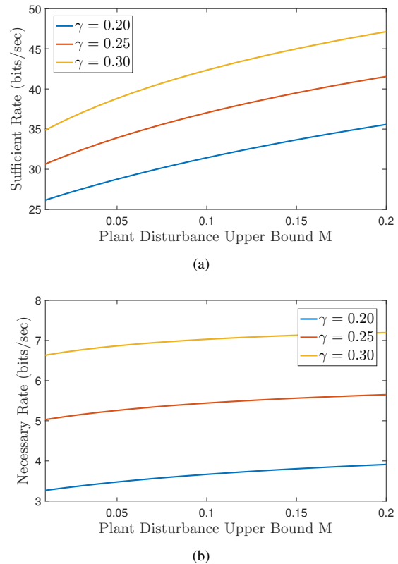
Fig. 9. (a) Sufficient and (b) necessary transmission rate vs plant disturbance upper bound M . Other simulation parameters are as follows: A = 5.5651 , b = 1.01 , \rho_0 = 0.1 , and J = (M/(A\rho_0))(e^{A\gamma} - 1) + 0.2 .
