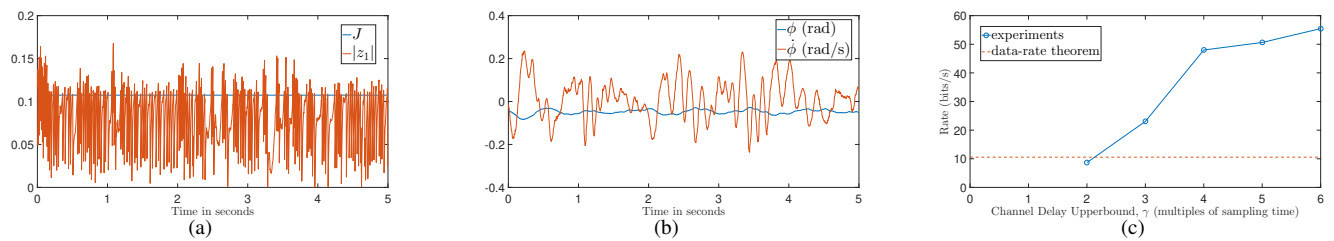
Fig. 7. Experimental results for controlling an inverted pendulum with the proposed event-triggered control strategy. (a) shows the triggering threshold J and the estimation error in the pendulum's angular position z_1 = \phi - \hat{\phi} , where \phi is the sensor measurement and \hat{\phi} is the estimate of the angular position. (b) shows the actual angular position and velocity of the pendulum, with the former staying close to zero degrees (the desired upright position). In (a) and (b) the delay upper bound is set to five sampling times of the system (which is equal to 0.015 seconds) and the packet size is found to be 7 bits. (c) shows the information transmission rate in the experiments compared with the entropy rate of the system. The rate calculated from the experiments does not start at zero because the minimum channel delay upper bound is equal to two sampling times (0.006 seconds). The entropy rate of the system is 10.56 bits/sec, while the minimum transmission rate for delay bound equal to two sampling times is 8.66 bits/sec.
