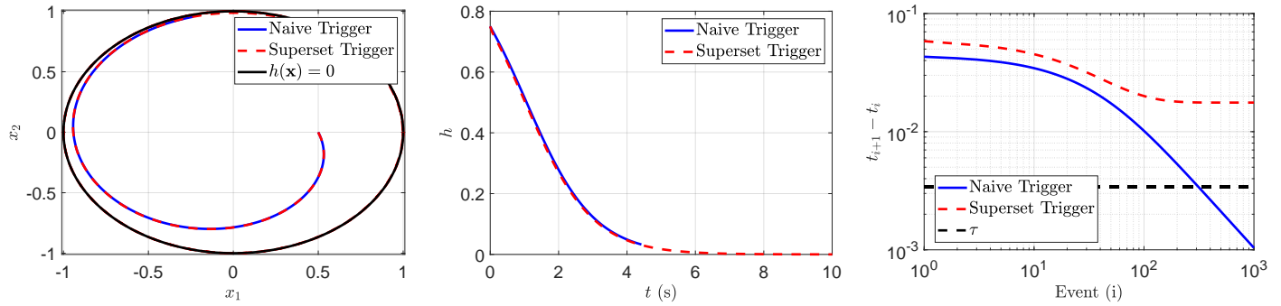
Fig. 2. Simulation results demonstrating safety achieved with an event-triggered controller. (Left) State trajectories for both triggers remain within the safe set for the length of the simulation. (Center) The value of the ISSf-BF h remains above zero for the length of the simulation, corresponding to the system remaining safe. (Right) The interevent times of the two trigger laws. The interevent times of the trigger law (21) decreases towards 0 as predicted by Lemma 1 while the trigger law (23) satisfies the theoretical bound.
