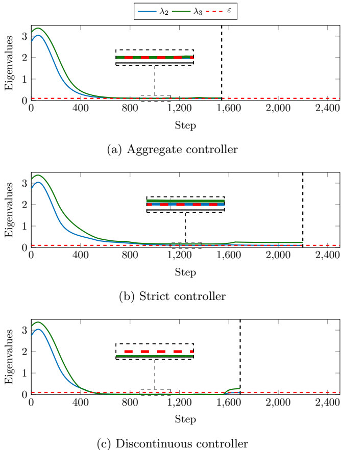
Fig. 1. Eigenvalue evolution during the simulations under the different controllers. The dashed black lines represent the end of the network task.
