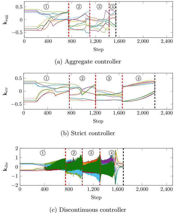
Fig. 2. Control inputs during the simulations of different controllers. We report all the components of the control input for each robot.
