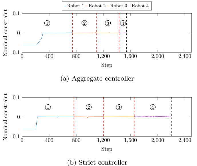
Fig. 3. Nominal constraint (17) during the simulations. The dashed red lines represent the instant in which the robot priority changes, due to the fact that a target has been reached. The number for each time slot corresponds to the robot with the highest priority.
